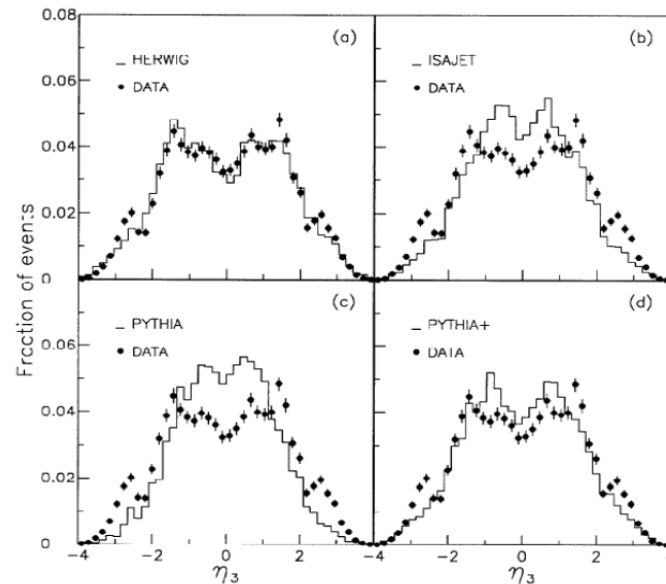
FIG. 13. Observed \eta_3 distribution compared to the predictions of (a) HERWIG; (b) ISAJET; (c) PYTHIA; (d) PYTHIA+.
